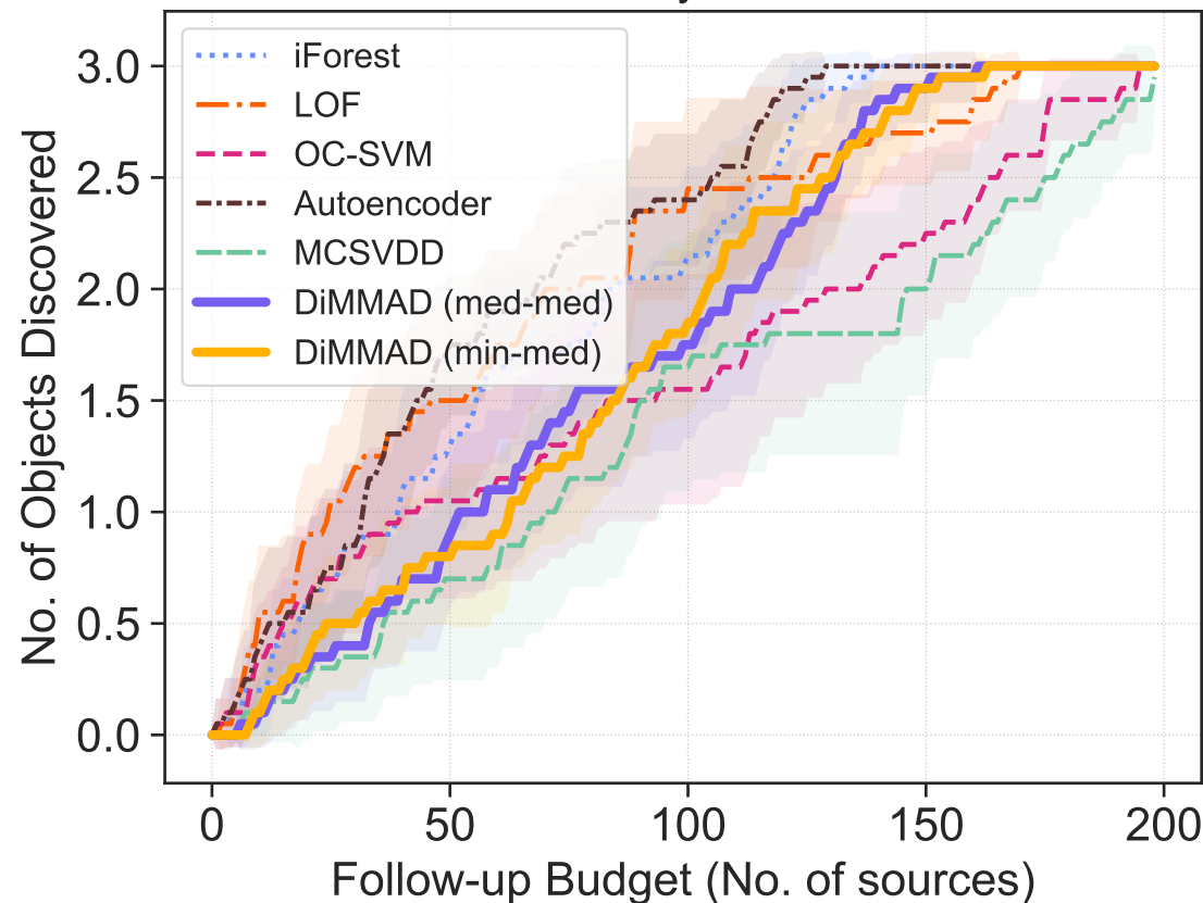
Anomaly: SLSN
